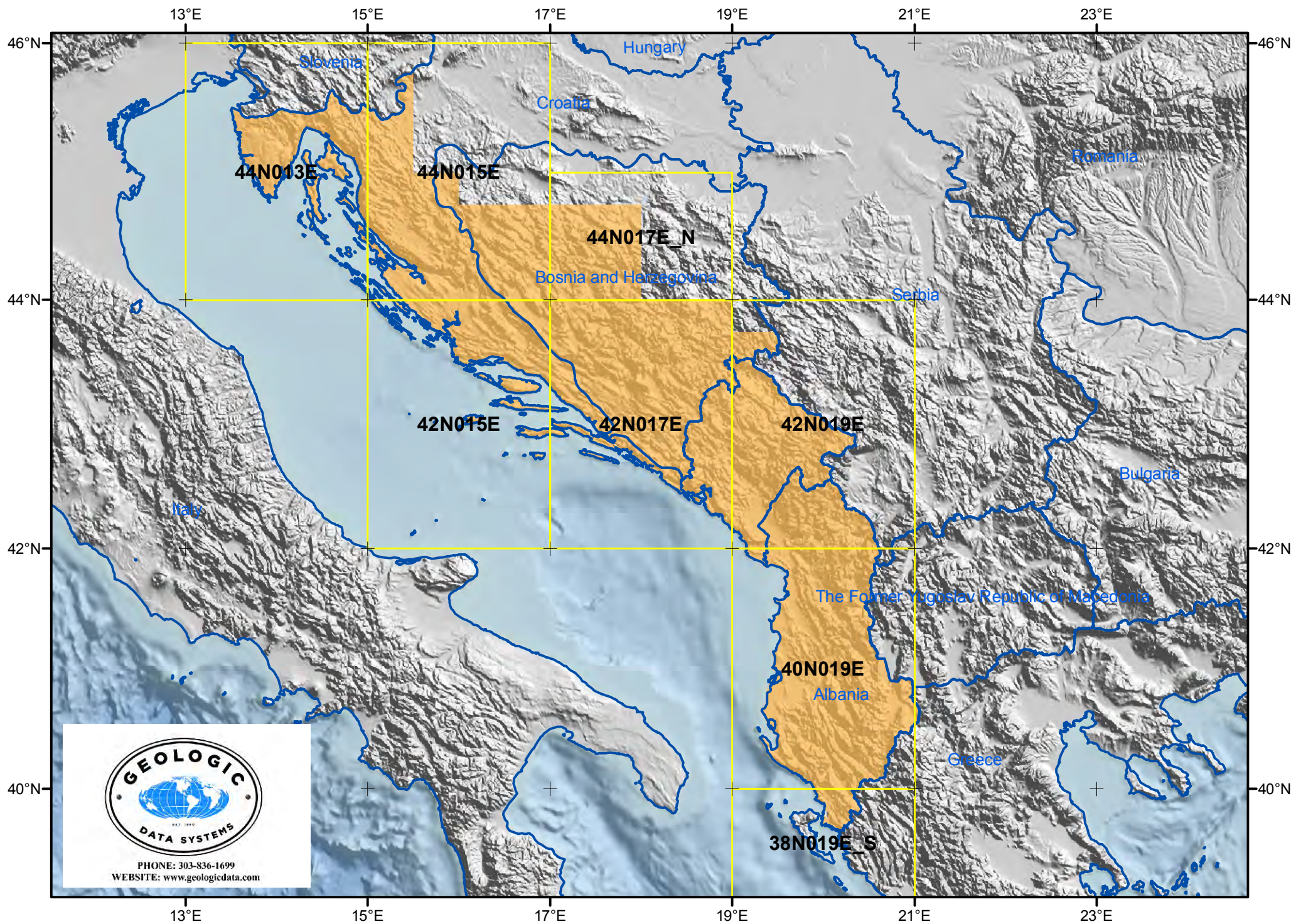
Index for the 1:200,000 scale Adriatic Region Geologic Mapping Project. Yellow outline shows 200,000 scale 2°x2° sheets, numbered based on the lower left coordinate.
