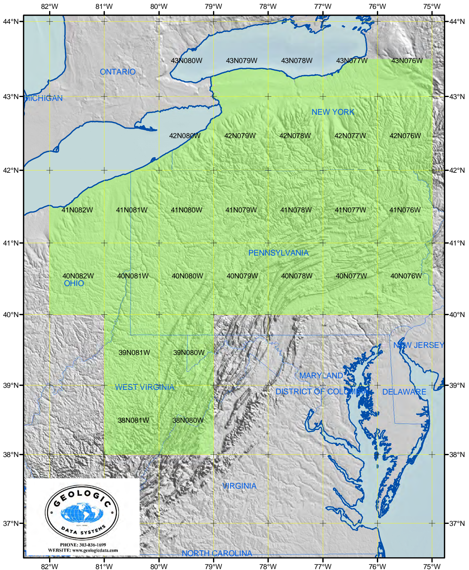
Index for the 1:100,000 scale Northern Appalachian Basin Region Geologic Mapping Project. Yellow outline shows 100,000 scale sheets numbered based on the lower left coordinate.
