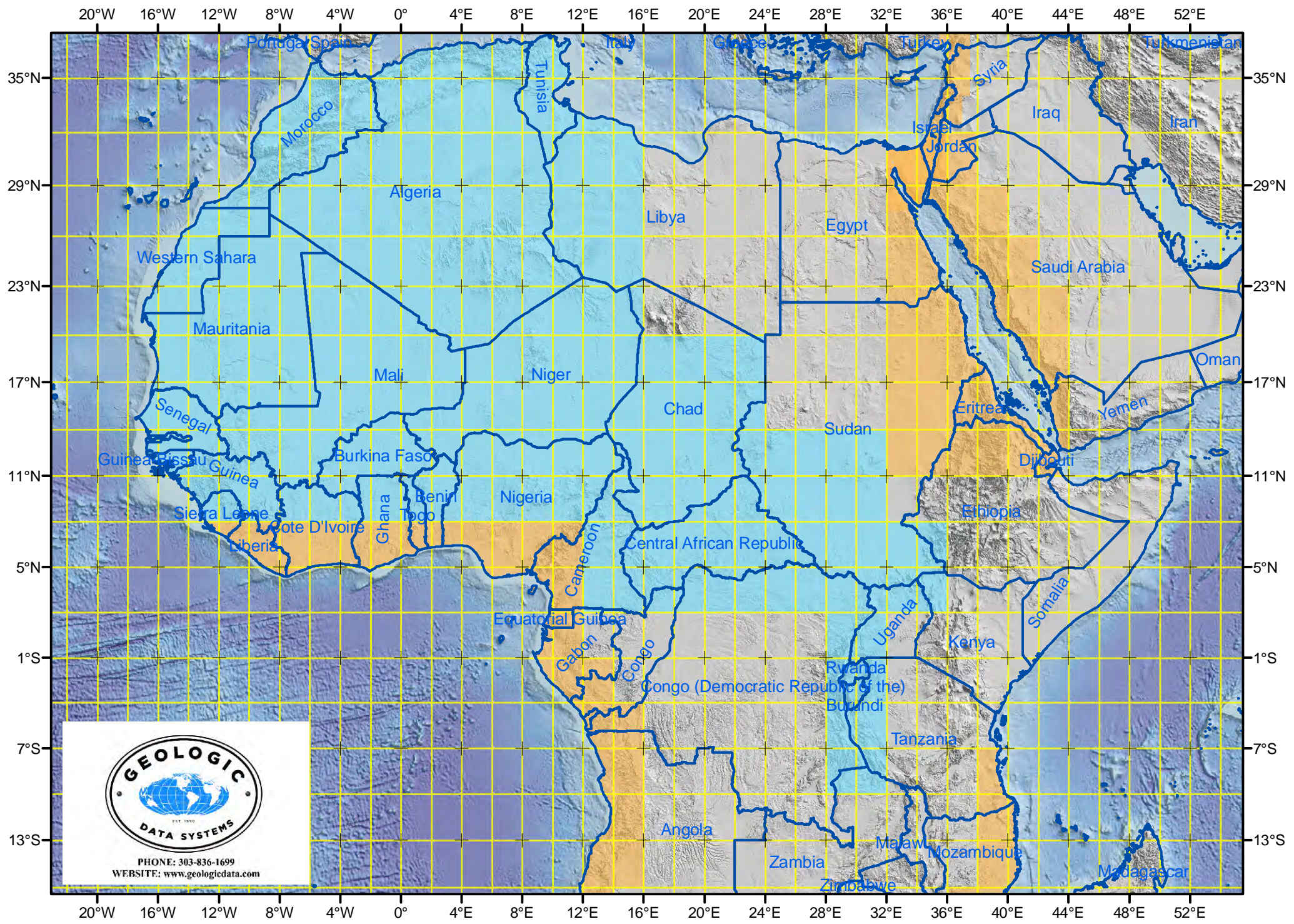
Index for the 1:500,000 (blue) & 1:250,000 (orange) scale North and Central Africa Geologic Mapping Projects. Yellow outline shows 250,000 scale sheets, numbered based on the lower left coordinate.
