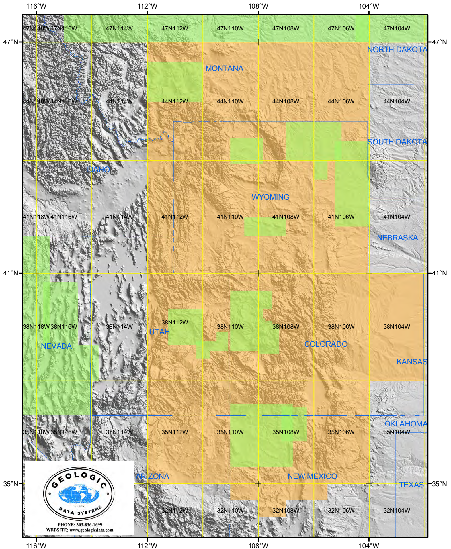
Index for the 1:250,000 scale Rocky Mountain Region Geologic Mapping Project (orange). Yellow outline shows 250,000 scale sheets, numbered based on the lower left coordinate; green areas are more detailed map projects.
