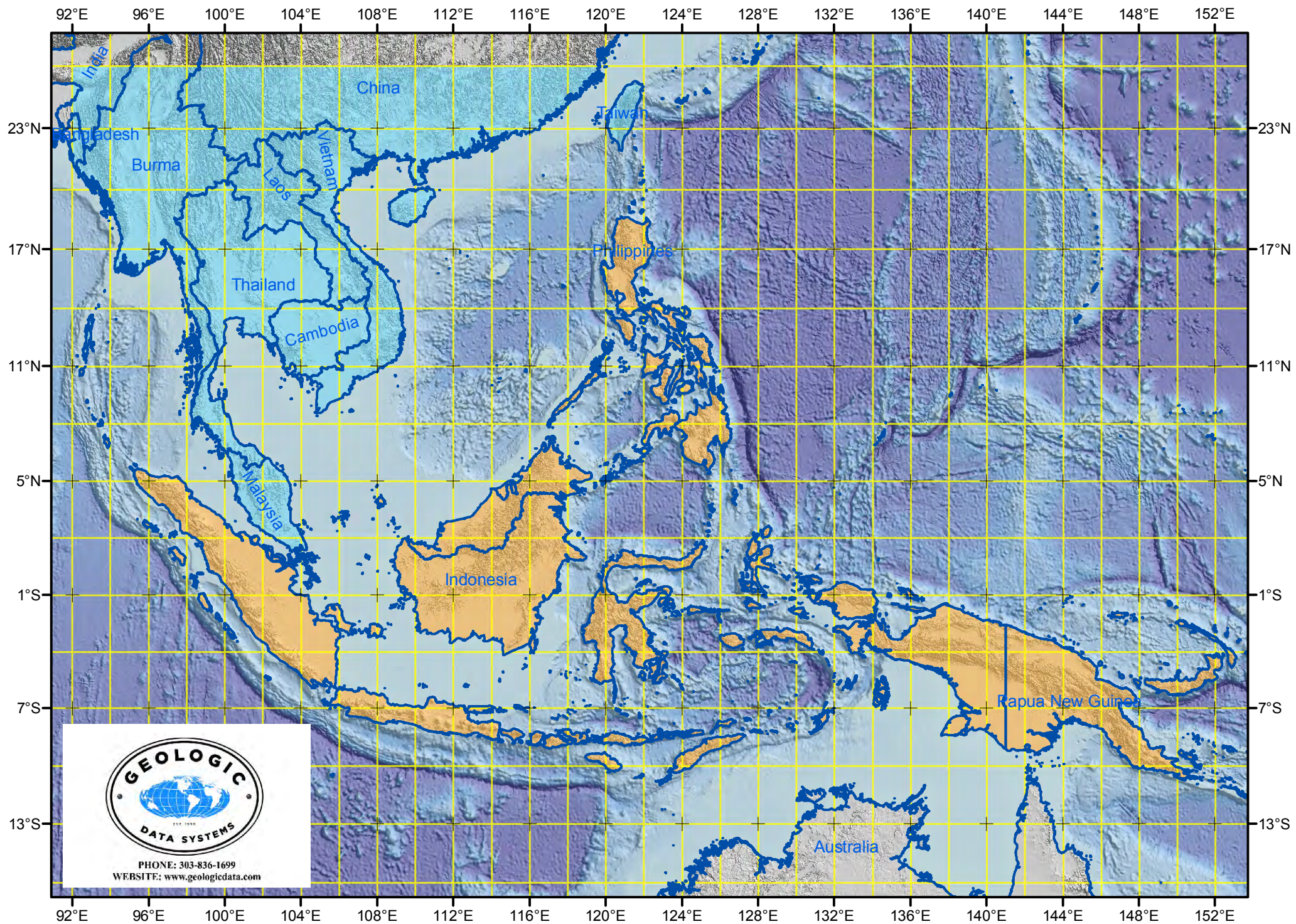
Index for the 1:500,000 (blue) & 1:250,000 (orange) scale SE Asia Geologic Mapping Project. Yellow outline shows 250,000 scale sheets, numbered based on the lower left coordinate.
